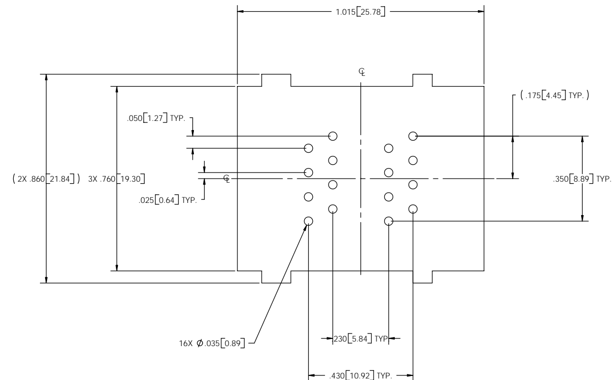
FOOTPRINT LOOKING DOWN THRU THE PART
