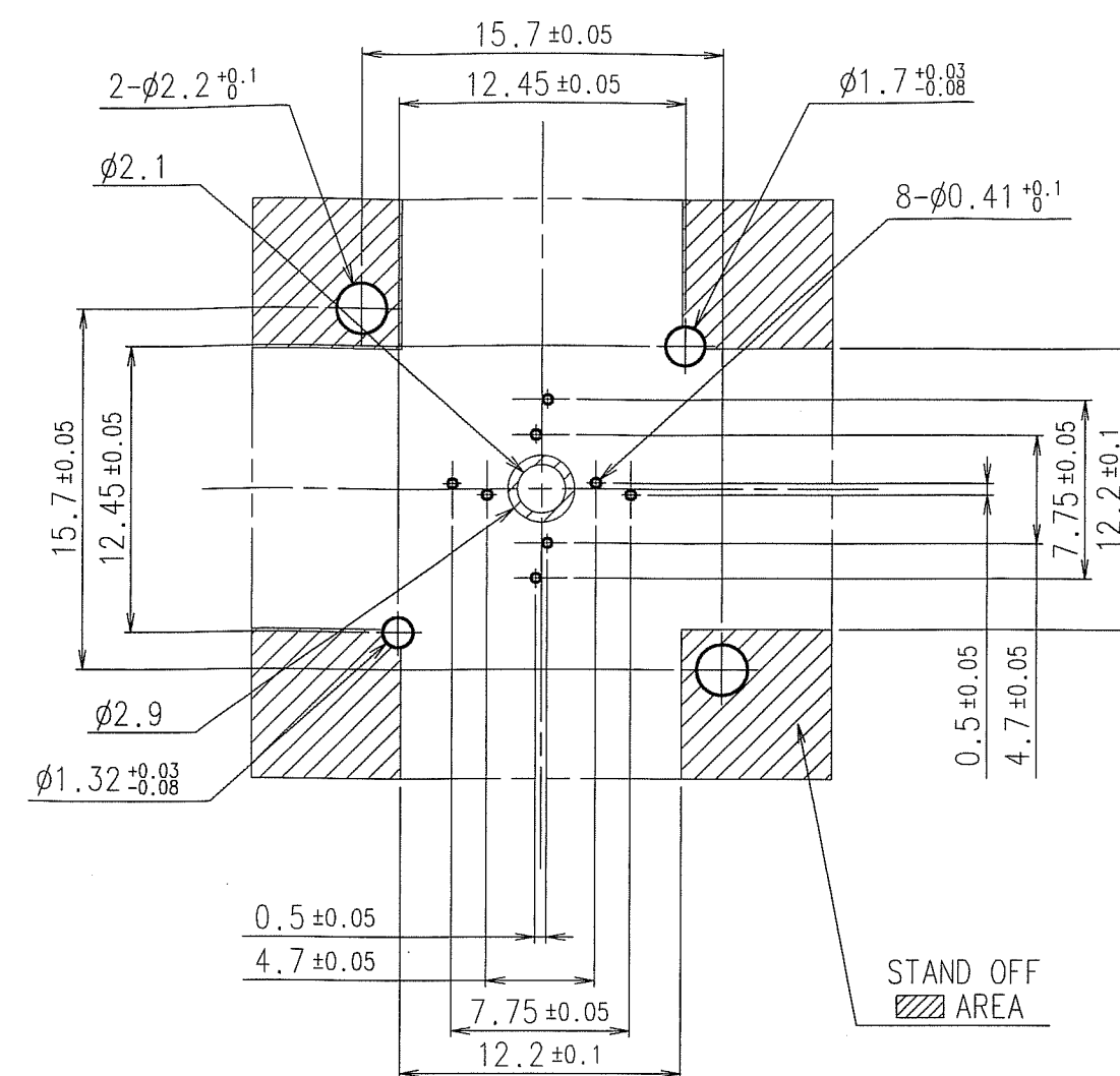
PCB PATTERN (TOP VIEW) (S=3:1)
