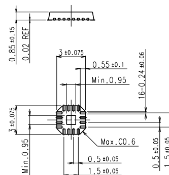
MATCHING DEVICE (S=5:1)
